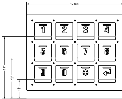
KEYPAD VERSION 3x4 VERSION W/ FULL-SIZED BUTTONS (3" SQ)
