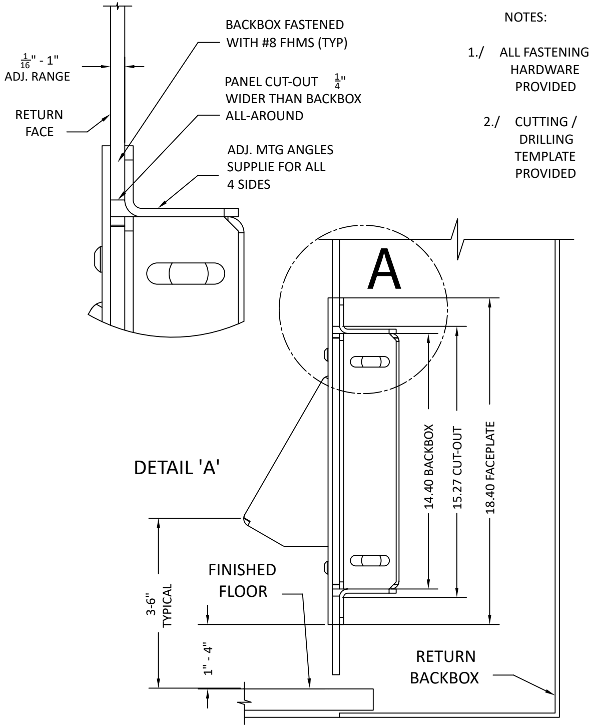
COP FLUSH-MTD - SECTION THRU FRONT RETURN / SWING PANEL
