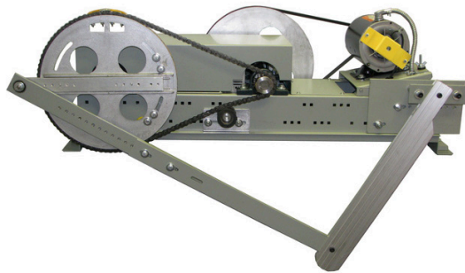
MOVFE-HH OPERATOR 115V W/ UNIVERSAL LENGTH DRIVE ARM (Side Slide Shown, Center Part Similar)
